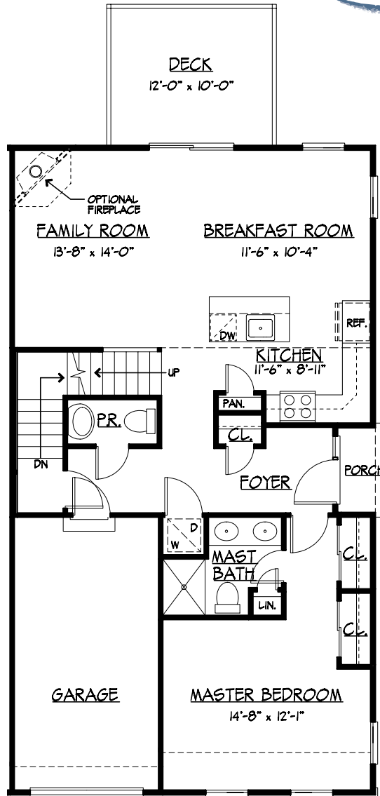
EASTON STANDARD FIRST FLOOR PLAN
