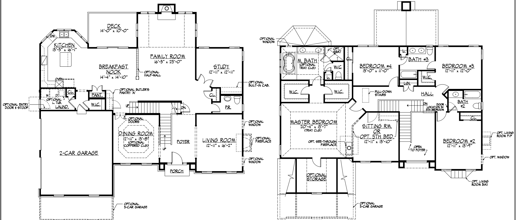
FIRST FLOOR PLAN "BROOKSHIRE" - CLASSIC
